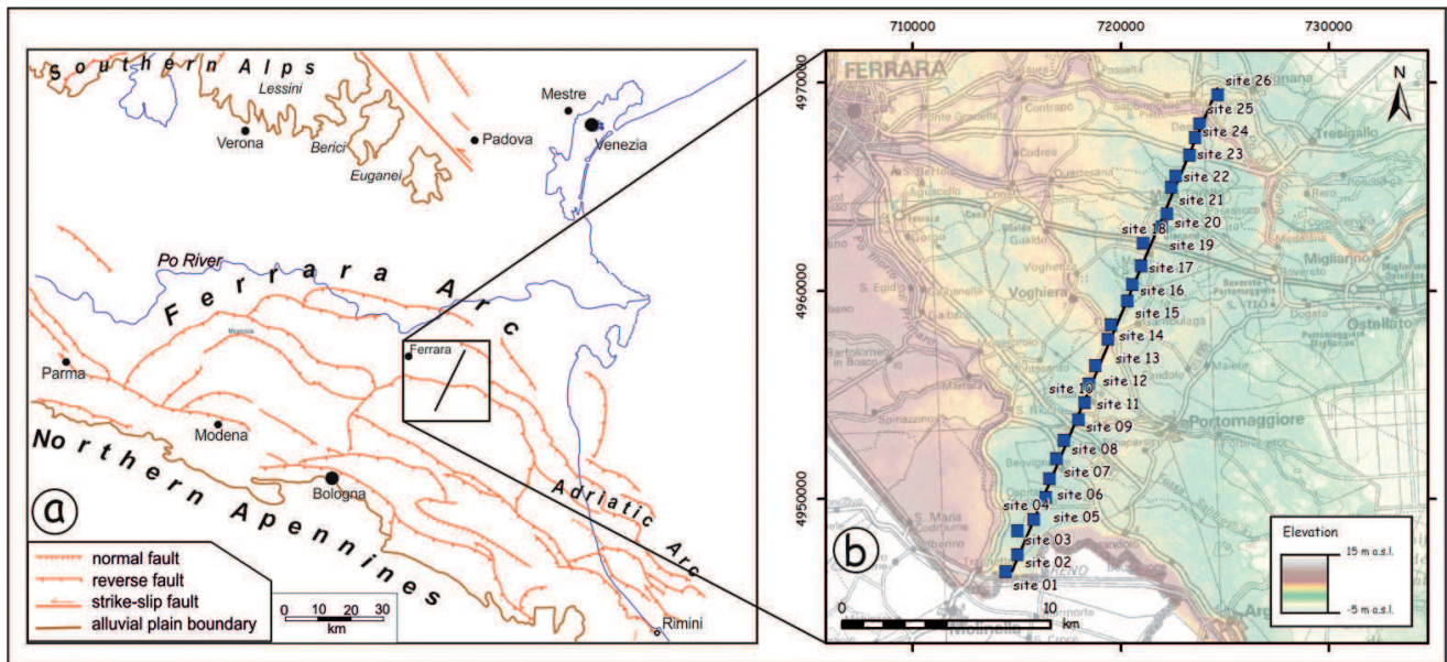
Fig. 1 – a) Simplified tectonic map of the blind northern Apennines showing the studied area [black boxes ESE of Ferrara: modified from CNR-PFG (1991)]. b) Location of the measured sites (blue dots) along investigated profile (black line).
